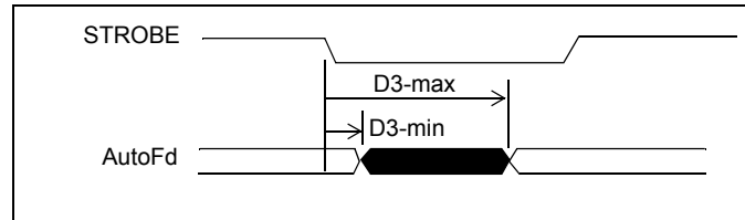
Figure 29 - Serial Interface Output Delay Timing
